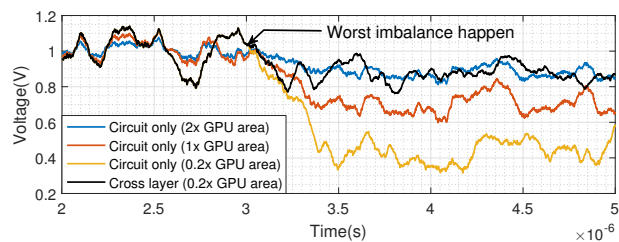
Fig. 9. Transient voltage waveforms under worst imbalance scenarios.
