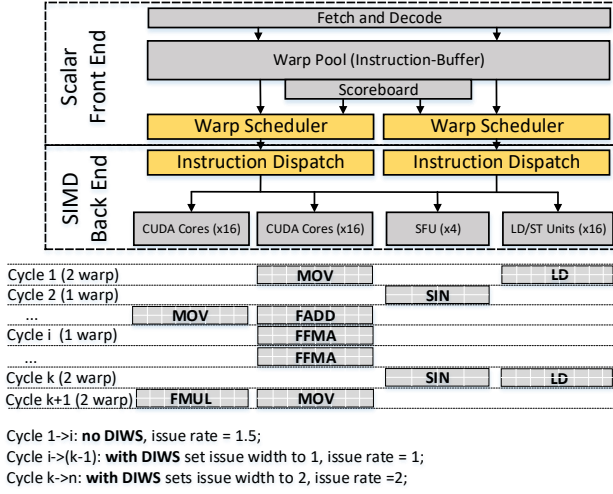
Fig. 6. SM microarchitecture and operation of dynamic issue width scaling. cycles k to n the issue width is back up to 2.
