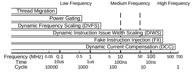
Fig. 5. Timescales of different power actuation mechanisms.
