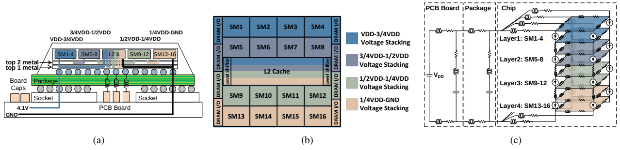
Fig. 1. Implementation of the voltage-stacked GPU system: (a) at the board level; (b) physical layout of the voltage-stacked domains on the die; (c) the corresponding electrical circuit model.
