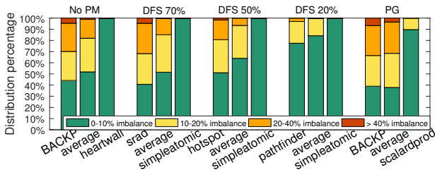
Fig. 17. Distribution of imbalanced currents by their normalized magnitudes when no power management (No PM), DFS with different performance goals, and power gating are applied in a VS GPU.
