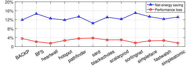
Fig. 14. Performance penalty and energy saving across benchmarks.
